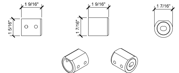
H PLTRACKFT RUBY SLIDING TUBE RUBY SLIDING DOORS (XO) SCALE: 6"=1'-0"
